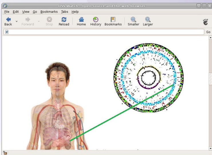
Web Application
