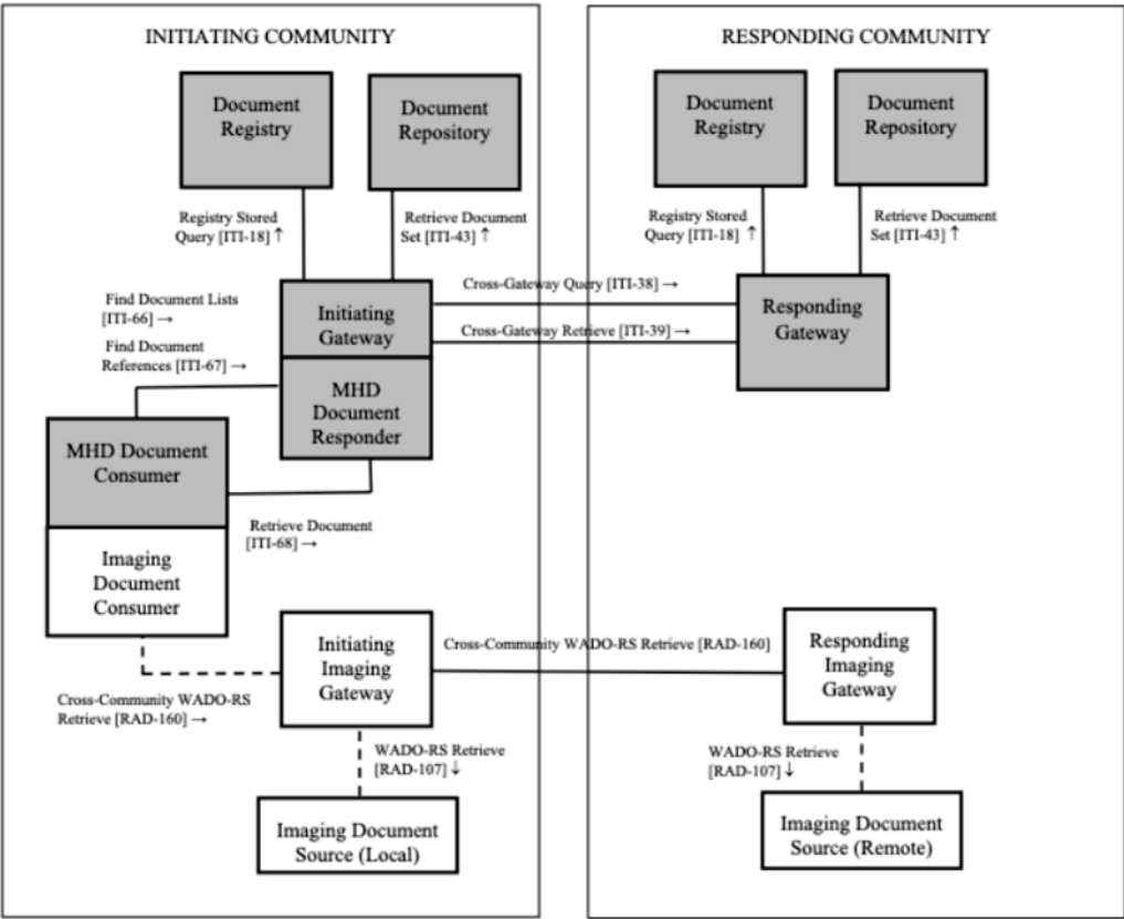
Figure 58.1-2: XC-WADO Actor Diagram (with MHD grouping)
