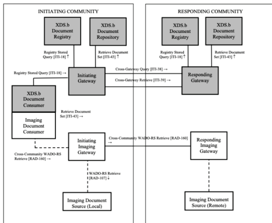
Figure 58.1-1: XC-WADO Actor Diagram (with XDS.b grouping)
