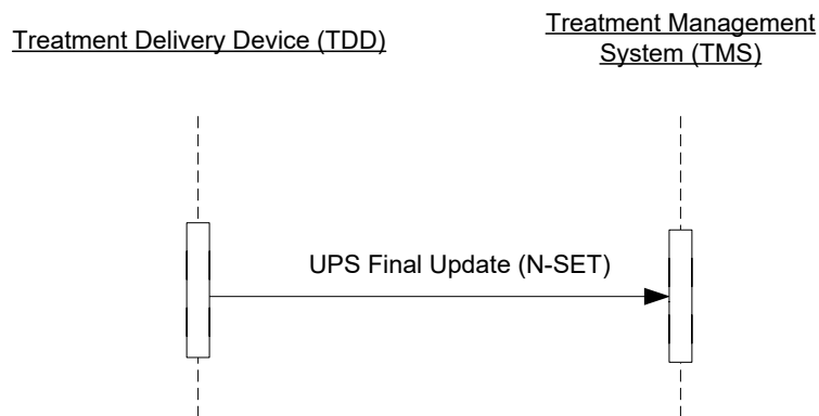
Figure 3.64.4-1: Interaction Diagram
