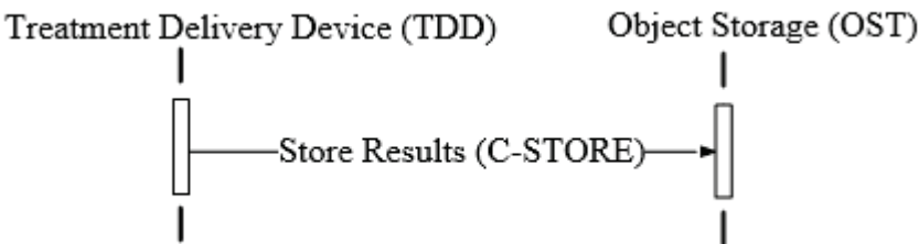
Figure 3.63.4-1: Interaction Diagram
