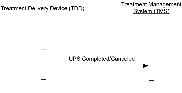
Figure 3.65.4-1: Interaction Diagram
