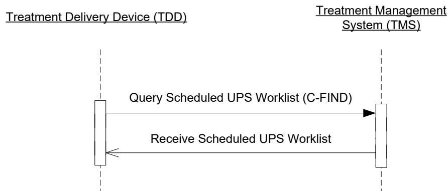
Figure 3.58.4-1: Interaction Diagram
