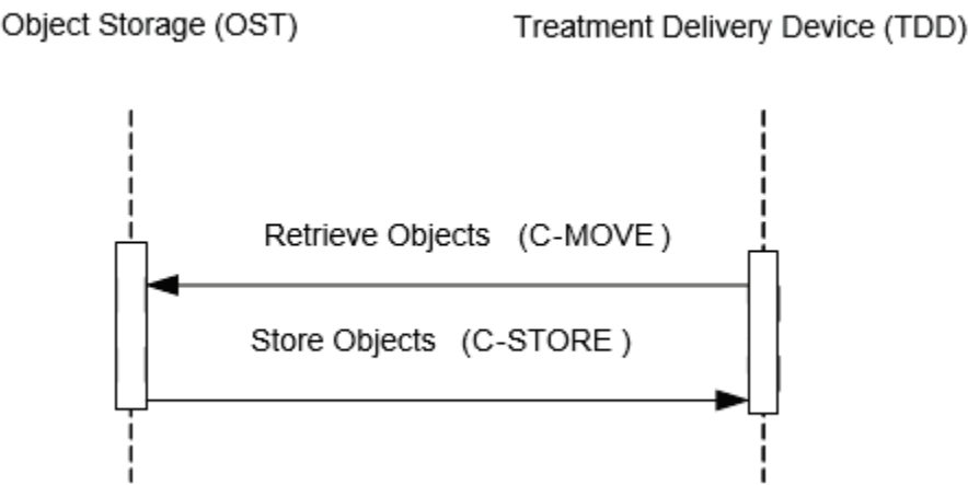
Figure 3.59.4-1: Interaction Diagram
