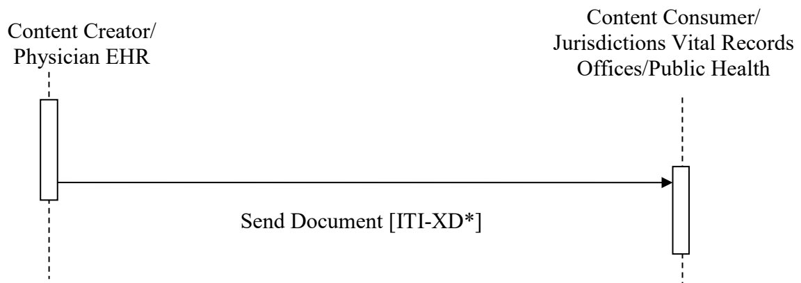
1615 Figure X.4.2.5.3-1: Use Case 5- EMR BFDR Document Submission
