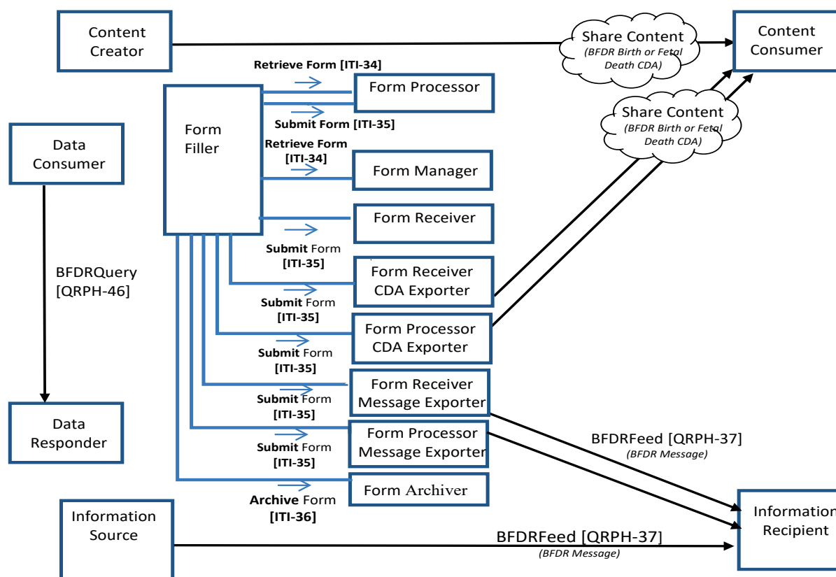
1155 Figure X.1-1: BFDR-E Actor Diagram
