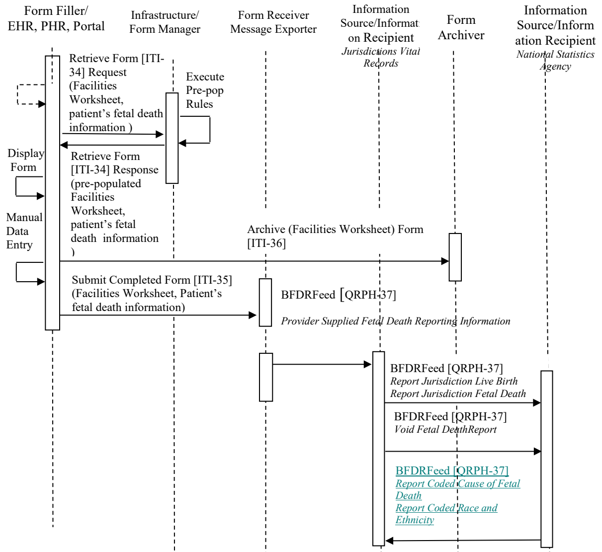
1510 Figure X.4.2.1.3-1: Use Case 1 - Forms Data Capture with Messaging
