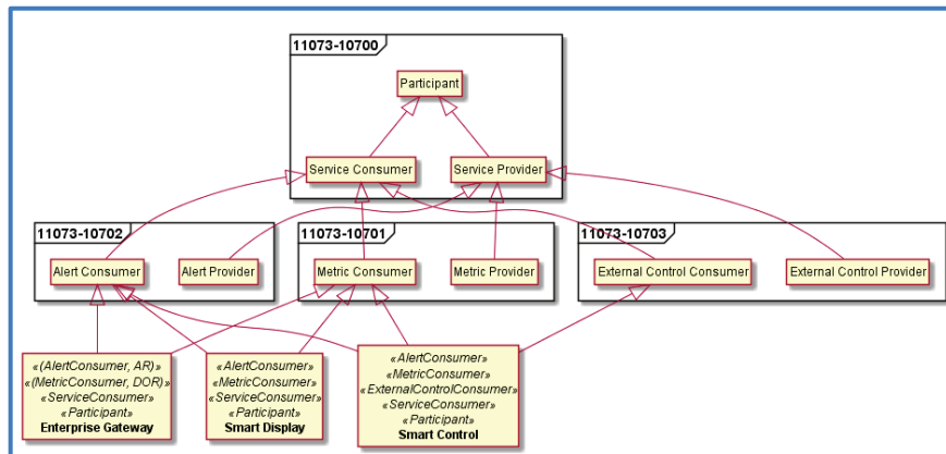
Figure 33 Example SDC Device Specialization – Gateway & "Smart" Devices
