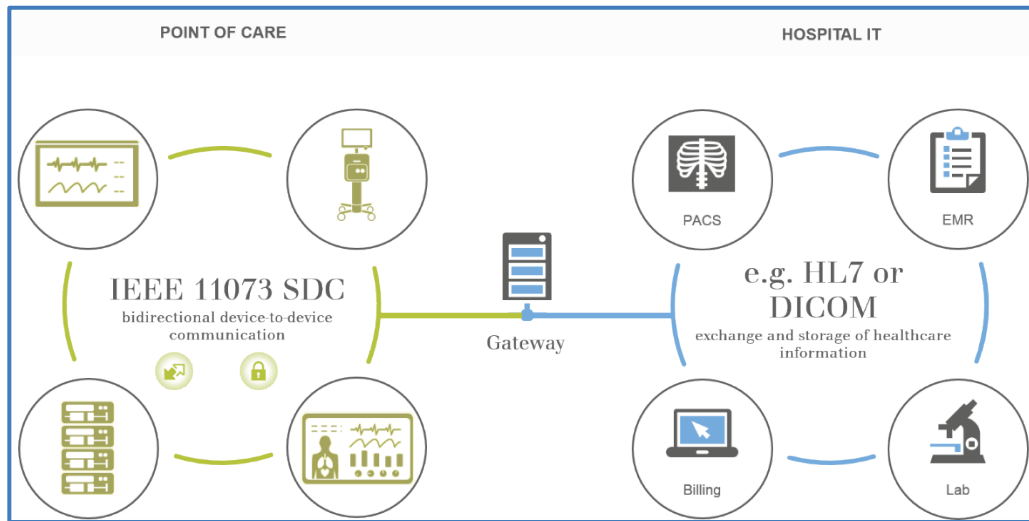
Figure 20 SDC Point-of-Care Gateway to Hospital Enterprise Systems
