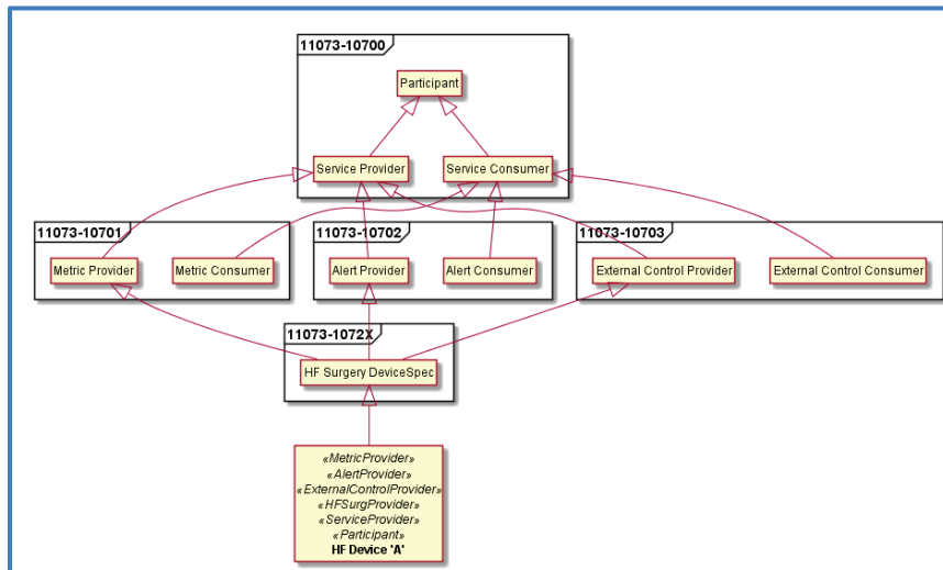
Figure 32 Example SDC Device Specialization - High-Frequency Surgery Device
