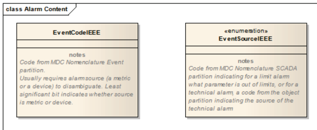
2995 Figure B.8.5-1: Event Identification Facet (Informative)
