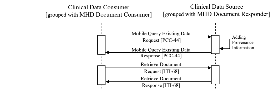
Figure X.4.2.2.2-1: Use Case #2 Process Flow in QEDm Profile
