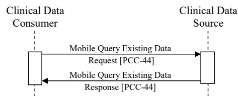
Figure X.4.2.1.2-1: Use Case #1 Process Flow in QEDm Profile
