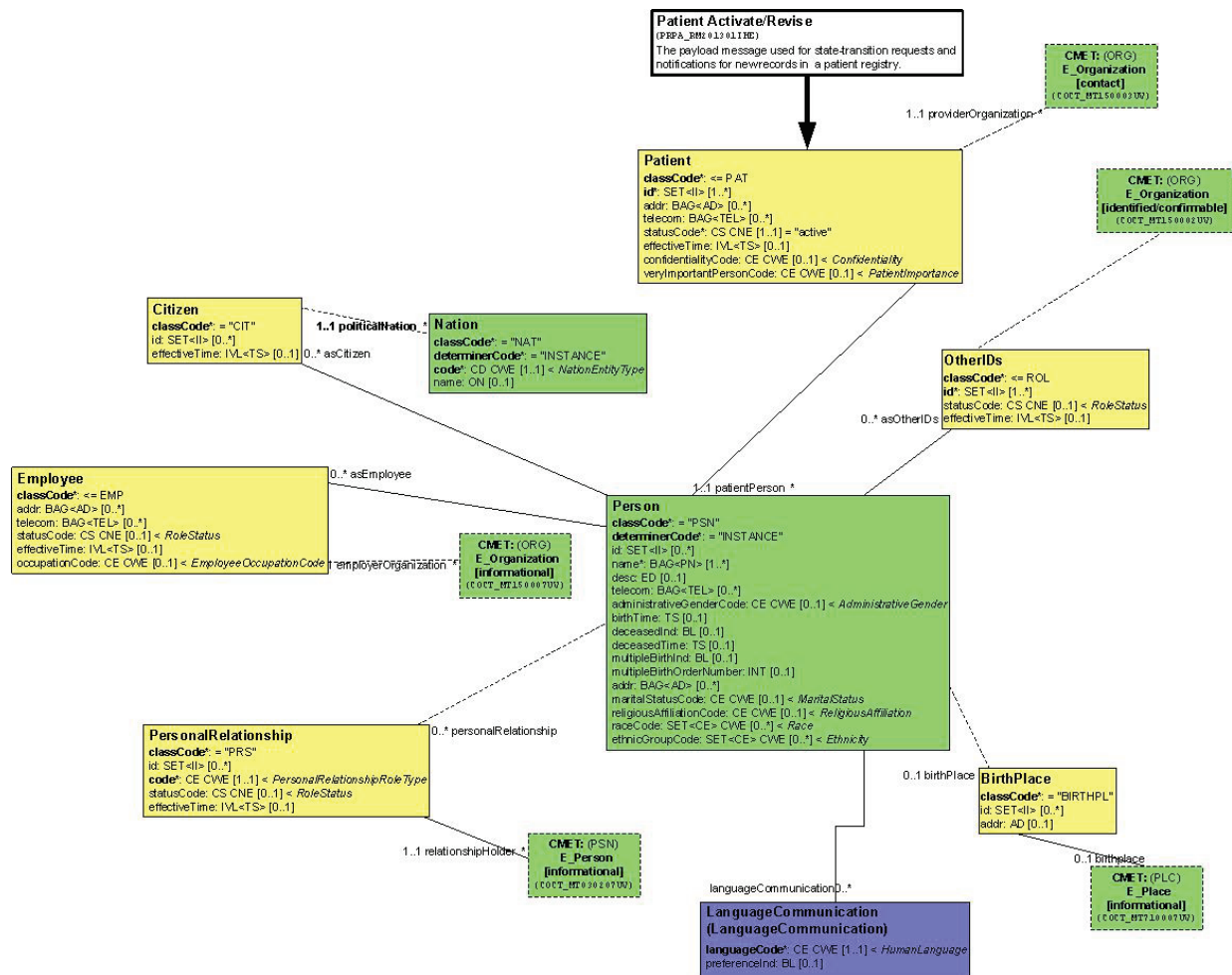
Figure 3.44.4.1.2.2-1: RMIM Diagram
