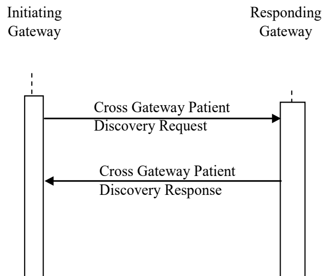
Figure 3.55.4-1: Interaction Diagram
