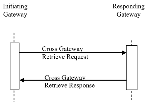
Figure 3.39.4-1: Interaction Diagram
