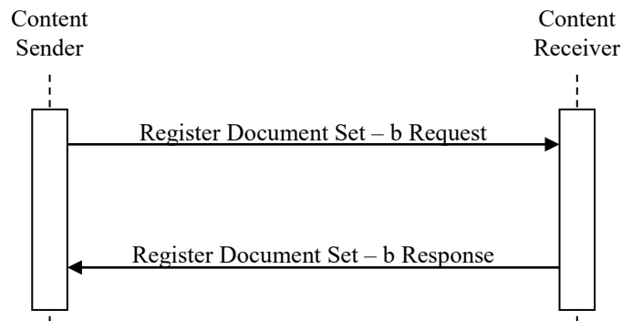
Figure 3.42.4-1: Interaction Diagram
