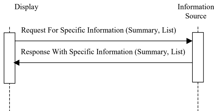
Figure 3.11.4-1: Request For Specific Information – Summary sequence
