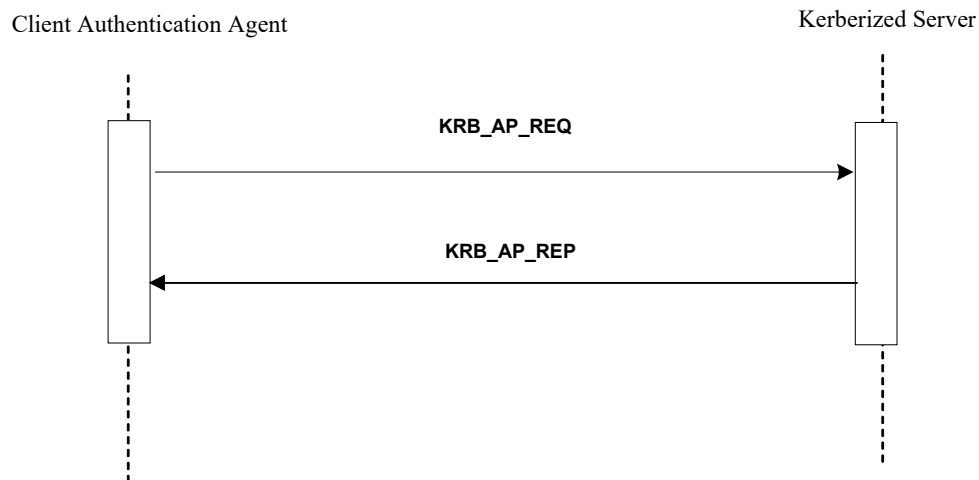
545 Figure 3.4-1: Kerberized Communications
