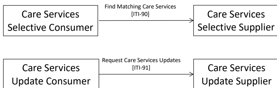
Figure 46.1-1: mCSD Actor Diagram
