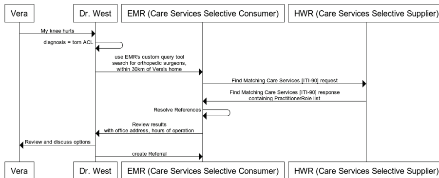
Figure 46.4.2.1.2-1: Provider Query Use Case
