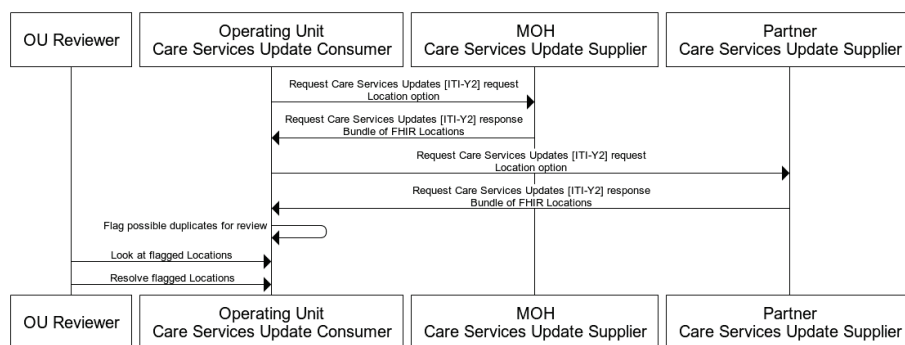
Figure 46.4.2.3.2-1: Cross-jurisdictional Site Management Workflow
