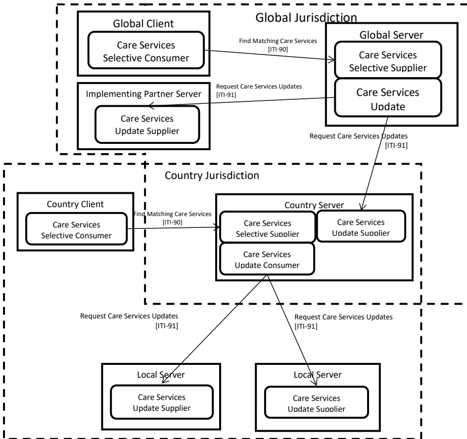
Figure 46.7.2-1: Federated and Cross Jurisdictional Deployment
