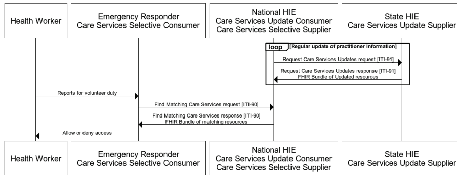
Figure 46.4.2.2.2-1: Federated Data Site Management Workflow
