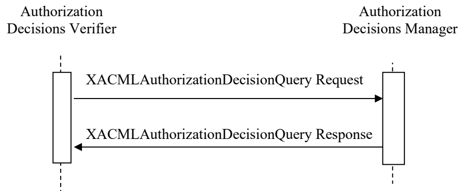
Figure 3.79.4-1: Interaction Diagram
