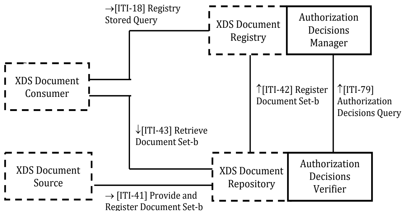
Figure 39.1-1: SeR Actor Diagram
