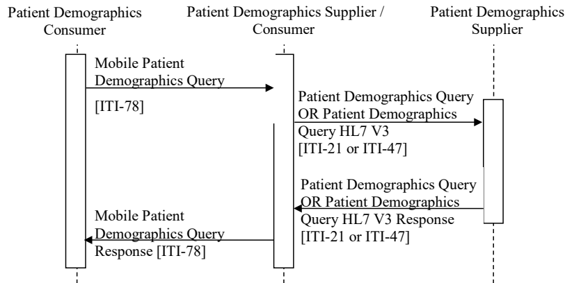
Figure 38.6-2: Sample PDQm gateway process flow
