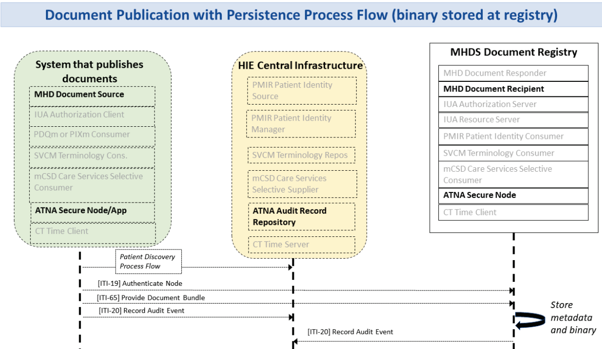
Figure X.1.1.1.1-1: Document Publication Process Flow
