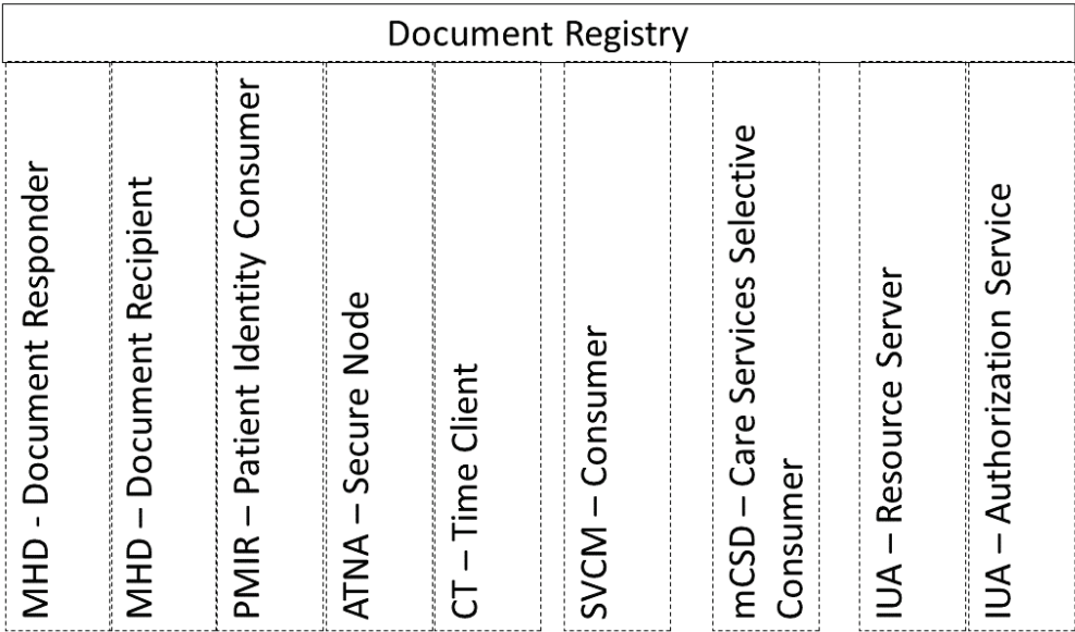
Figure X.1-1: MHDS Registry Actor Diagram
