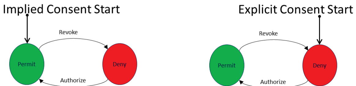
Figure X.2.2-2: Simple Consent state diagram
