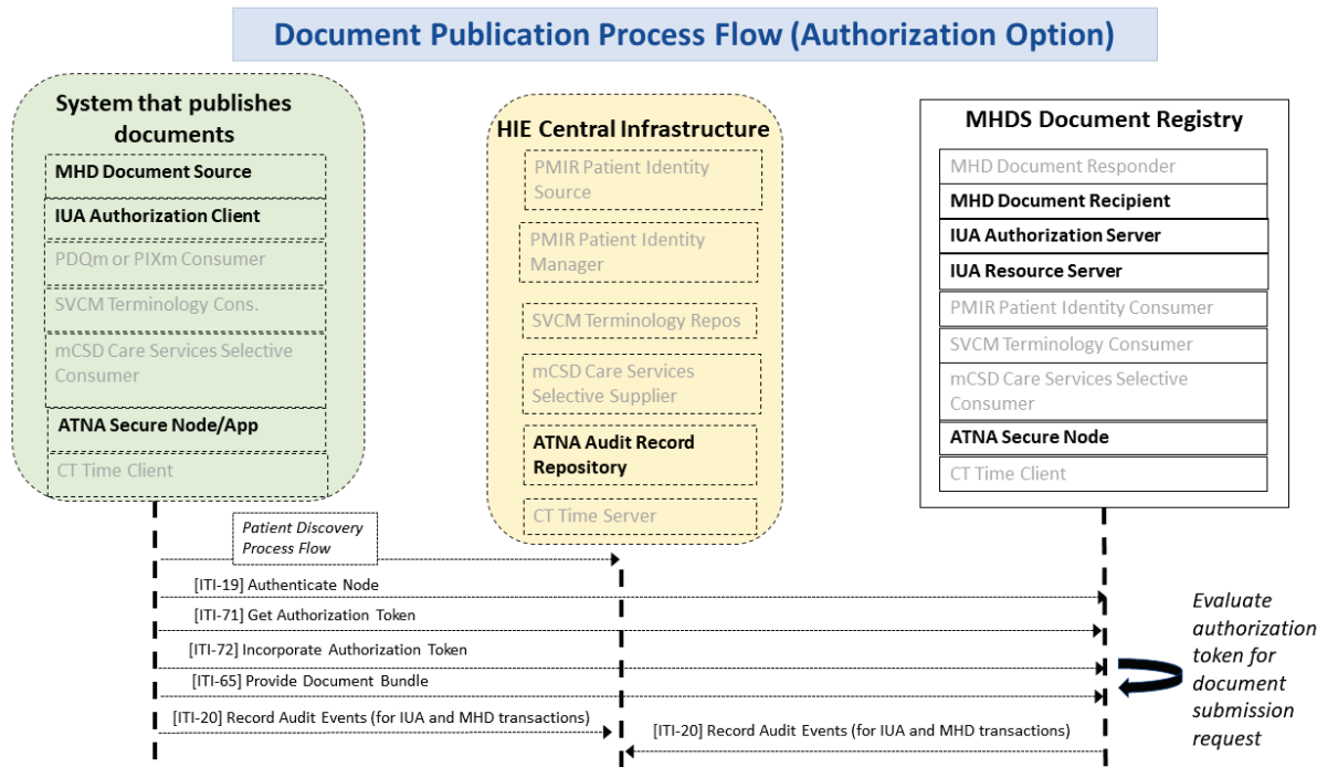
Figure X.2.1-1: Document Publication Process Flow with Authorization Option
