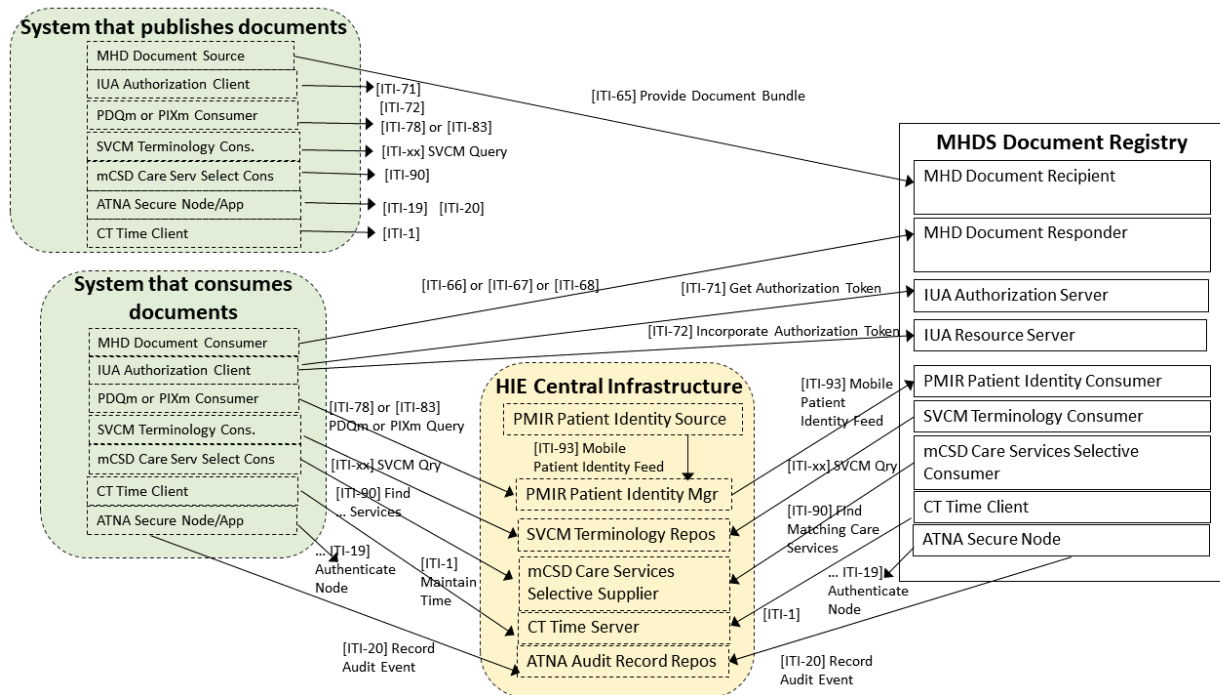
Figure X.1-2: MHDS Document Sharing Community
