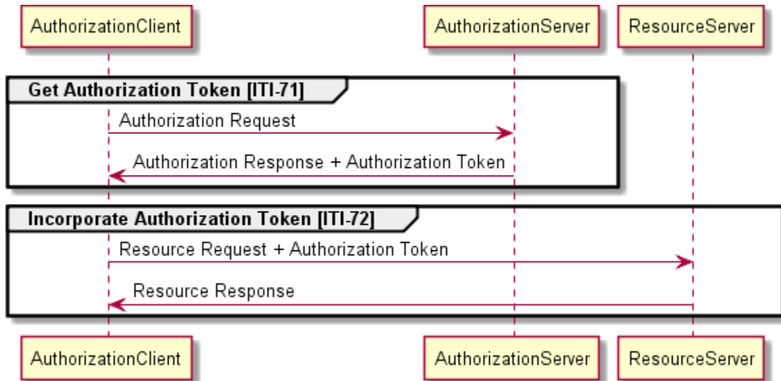
Figure 3.71.4-1: Basic Process Flow for Obtain HTTP RESTful Authorization and Incorporate Authorization Token Transaction
