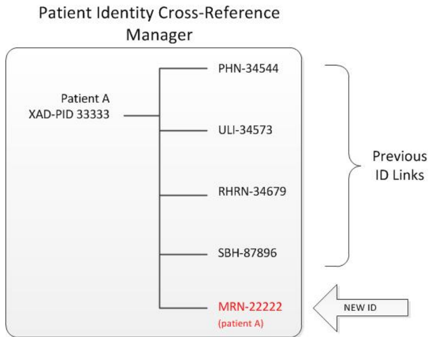
Figure 31.4.1-1. Local Patient Added to the Patient Identity Cross-Reference Manager
