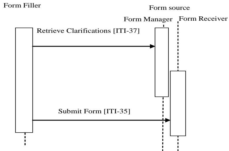
Figure 17.4-5: Case 5: Form Filler supporting Data Clarifications Option
