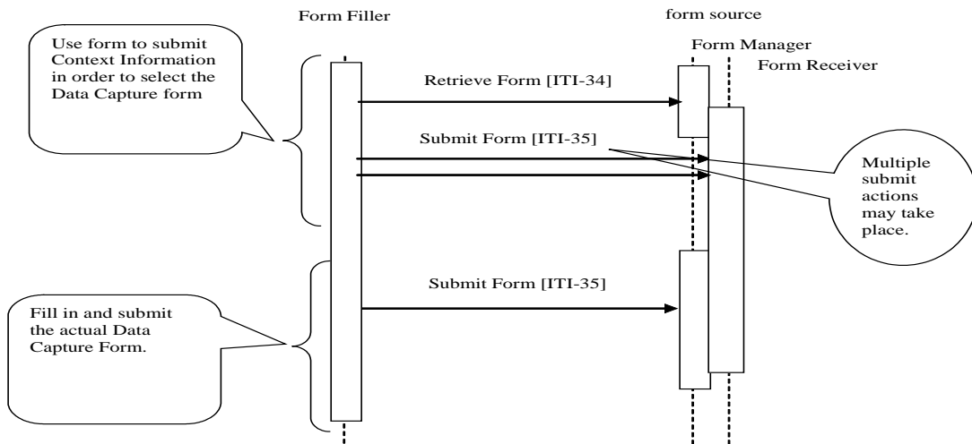
Figure 17.4-4: Case 4: Retrieve Form; Submit Form
