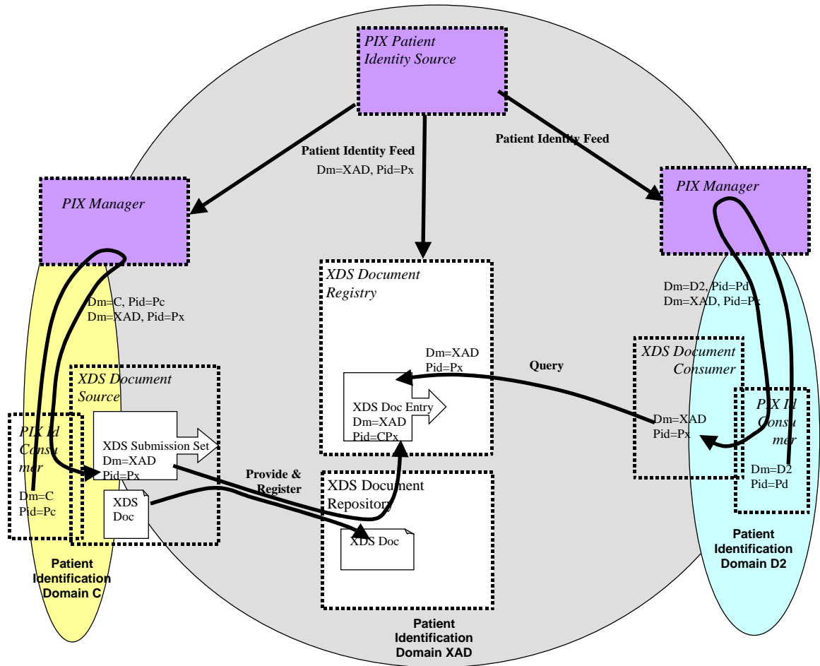
7030 Figure E.3-1: XDS Affinity Domain with patient ID cross-referencing with IHE PIX Managers
