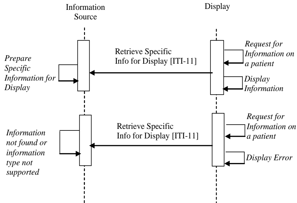
1110 Figure 3.3-1: Case 1: Retrieve Specific Information for Display Process Flow
