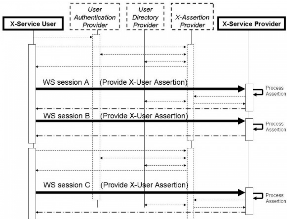
Figure 13.6-1: Cross-Enterprise User Assertion Process Flow
