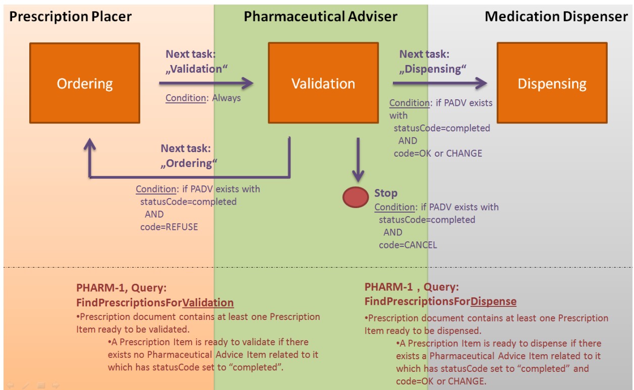
440 Figure 4.4.1-1 Scenario 1: Overall context of the workflow
