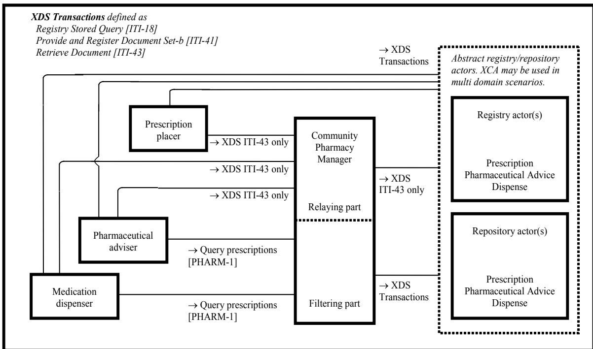
Figure 4.1-1 Community Medication Prescription and Dispense Actor Diagram
