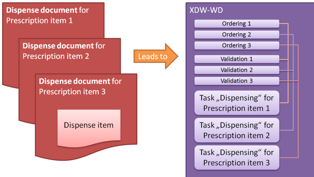
Figure 4.1.3.3-1: Prescription items leading to workflow tasks “Dispensing”
