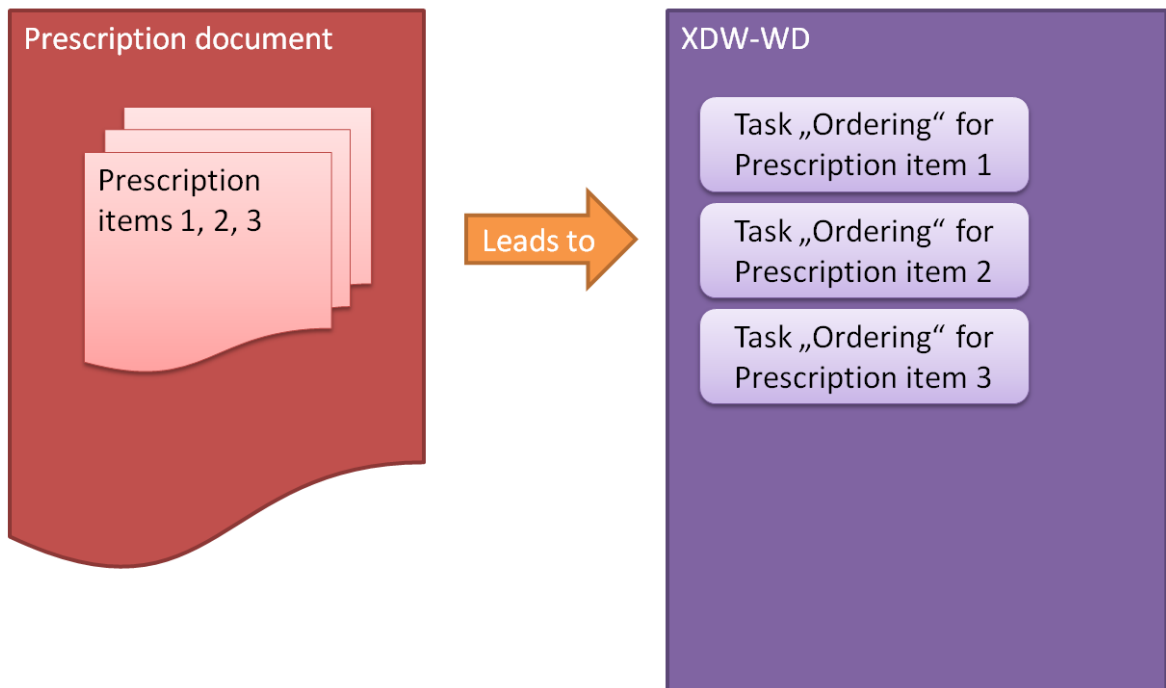
Figure 4.1.3.1-1 Prescription containing Prescription items leading to workflow tasks “Ordering”
