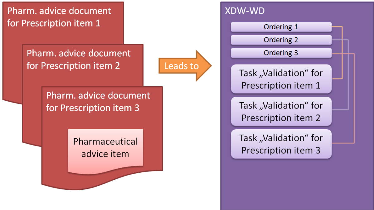
Figure 4.1.3.2-1 Prescription items leading to workflow tasks “Validation”
