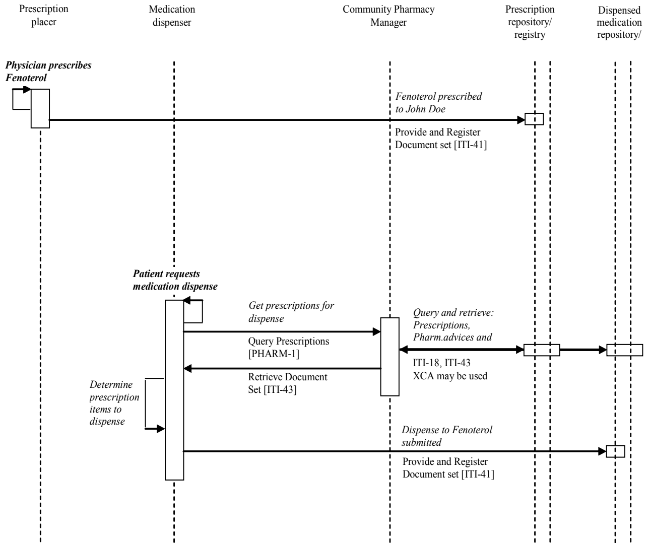
Figure 4.3.1.2-1 Use Case community pharmacy-active substance, publish & pull - Process Flow (Scenario 2: “Not including validation step”)
