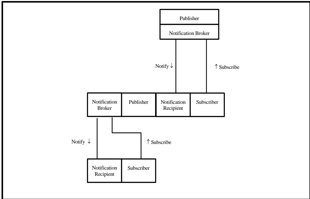
Figure 4.4.1-5 Cascading Notifications
