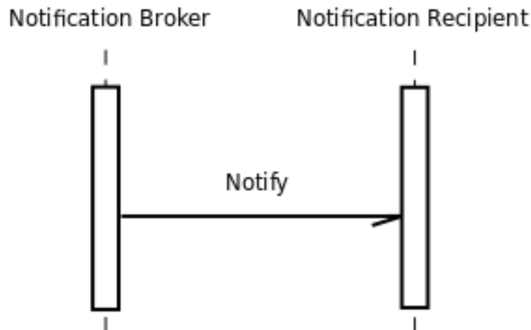
Figure 4.4.2.2.4-1: Notify Sequence
