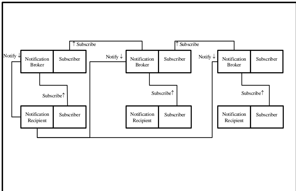
Figure 4.4.1-6 Cascading Subscriptions
