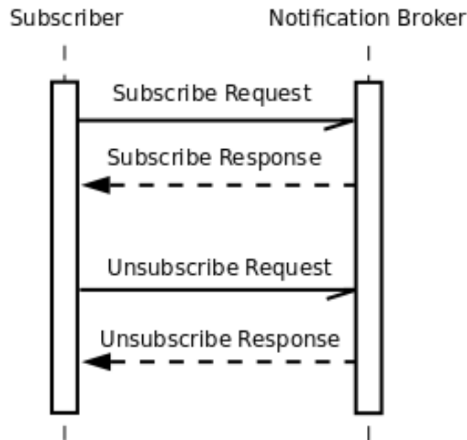
Figure 4.4.2.1.4-1: Subscribe Sequence
