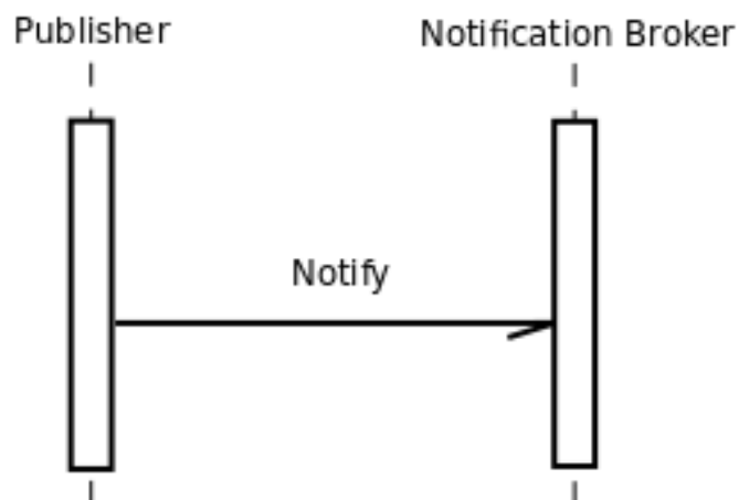
Figure 4.4.2.3.4-1: Publish Sequence
