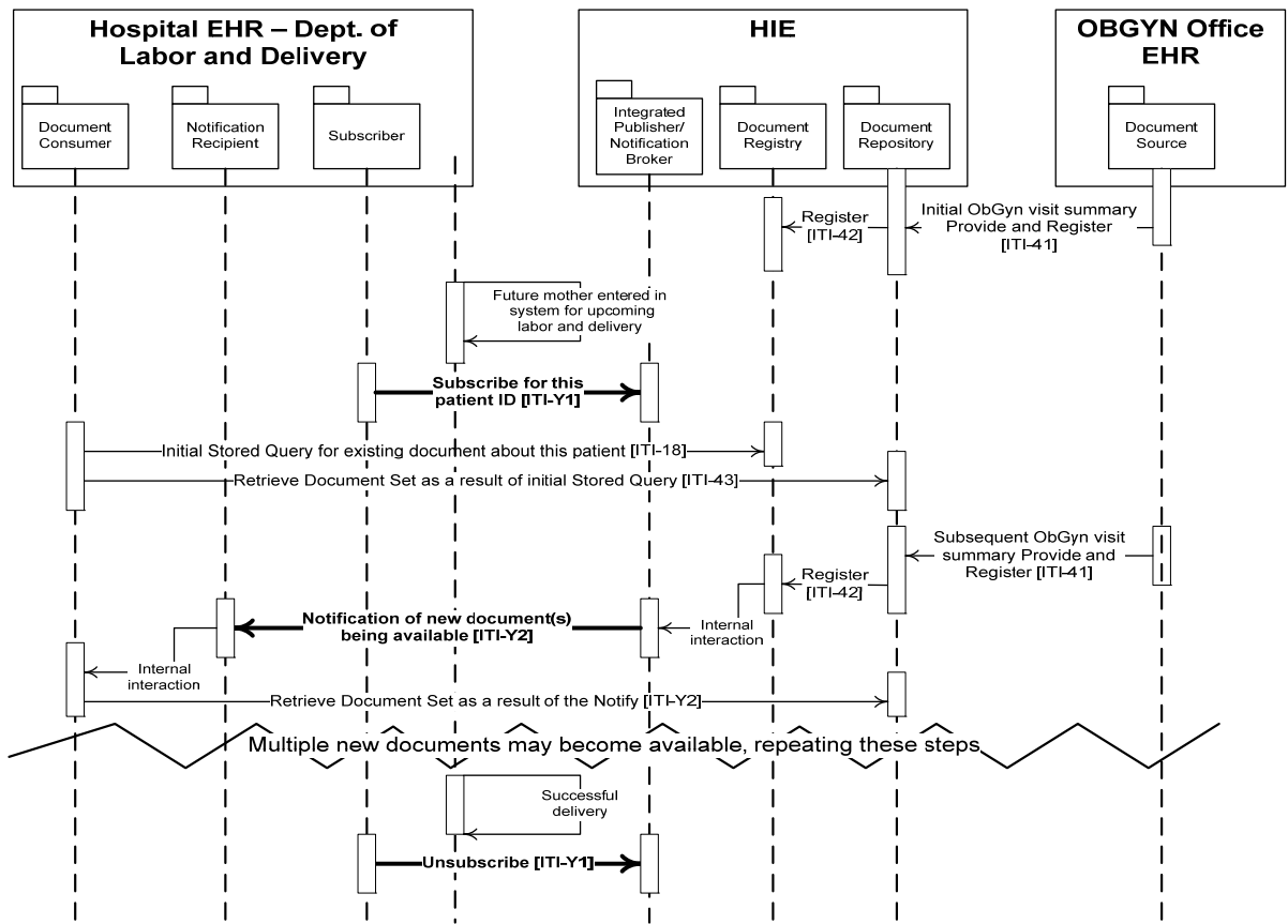
Figure 26.4-3: Interaction diagram
