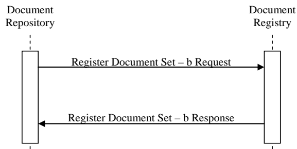
Figure 3.42.4: Interaction Diagram
