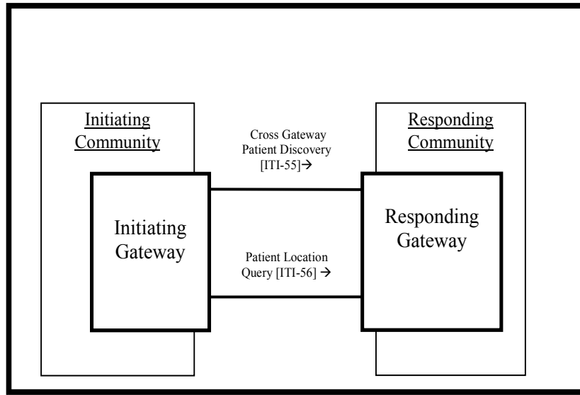
Figure 27.1-1 XCPD Actor Diagram
