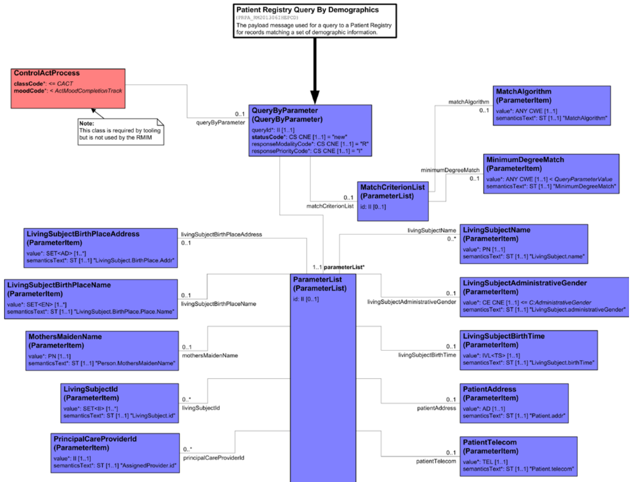
Figure 3.55.4.1.2-1 Patient Registry Query by Demographics Message
