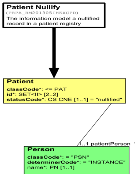
1305 Figure 3.55.4.3-1 Patient Nullify Message
