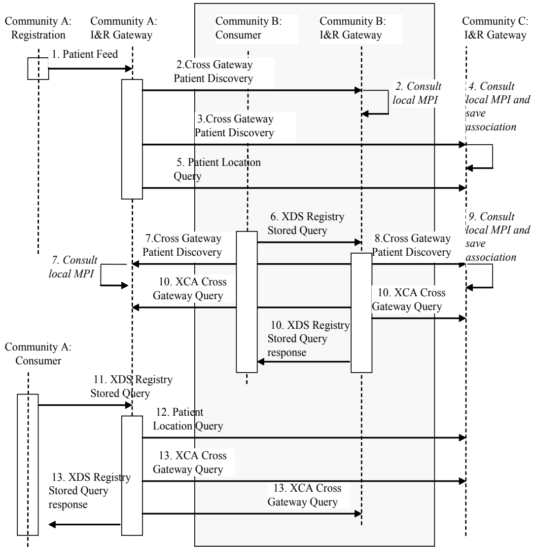
Figure 27.3.2.1-2 Detailed Interactions Health Data Locator (Informative)
